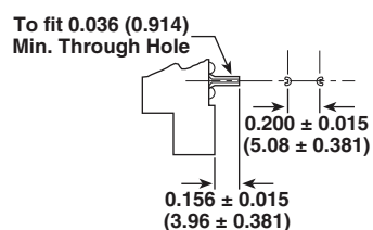
Type "L" Solder Dip
