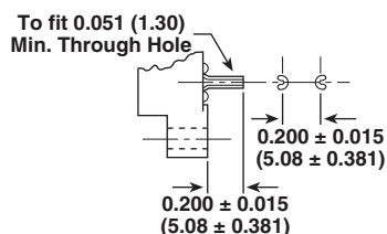
Type "K" Solder Dip
