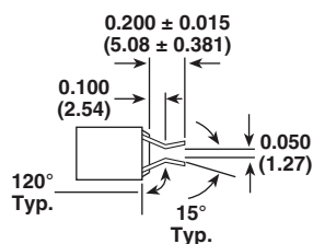
Type "E" Card Extender
