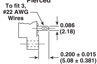
Type "A" Pierced
