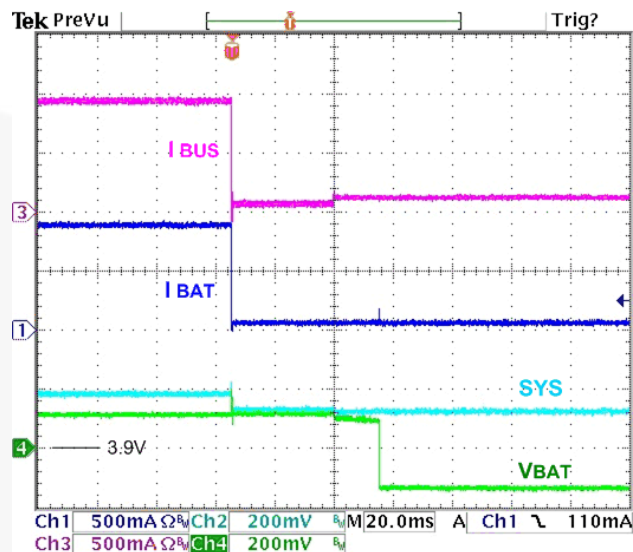
Figure 16. Battery Removal / Insertion while Charging, TE=1 , 3.9\text{ V}_{BAT} , I_{CHRG}=950\text{ mA} , I_{BUSLIM}=\text{No Limit} , 50\ \Omega SYS Load
