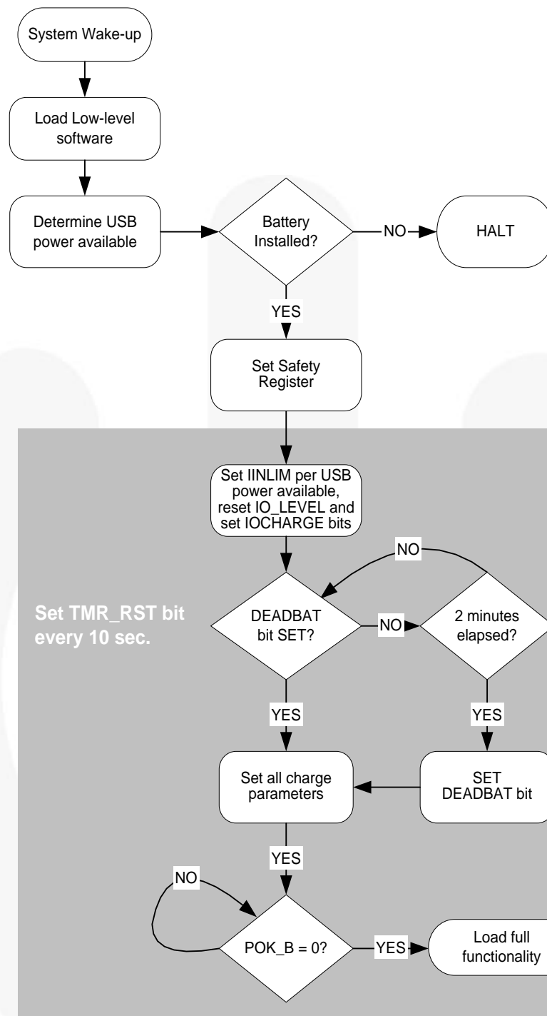
Figure 37. Recommended Host Software Sequence when Booting with Dead Battery
