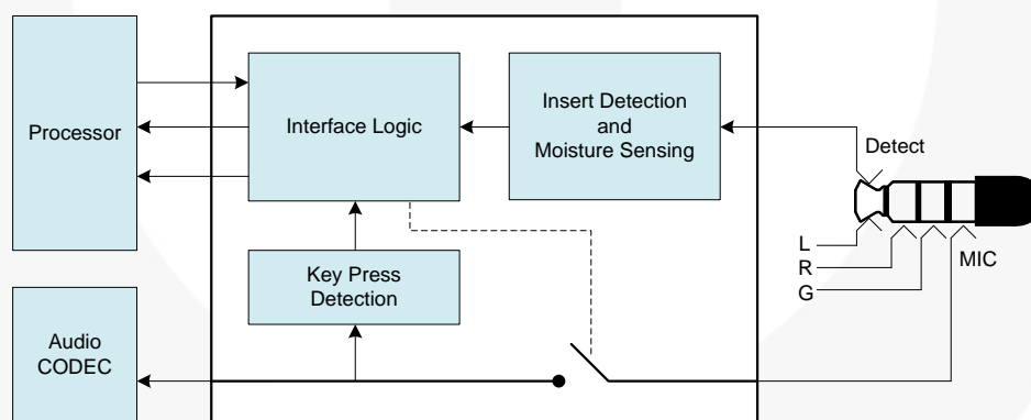
Figure 1. Block Diagram
