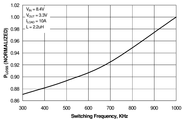
Figure 6. Power Loss vs. Switching Frequency
