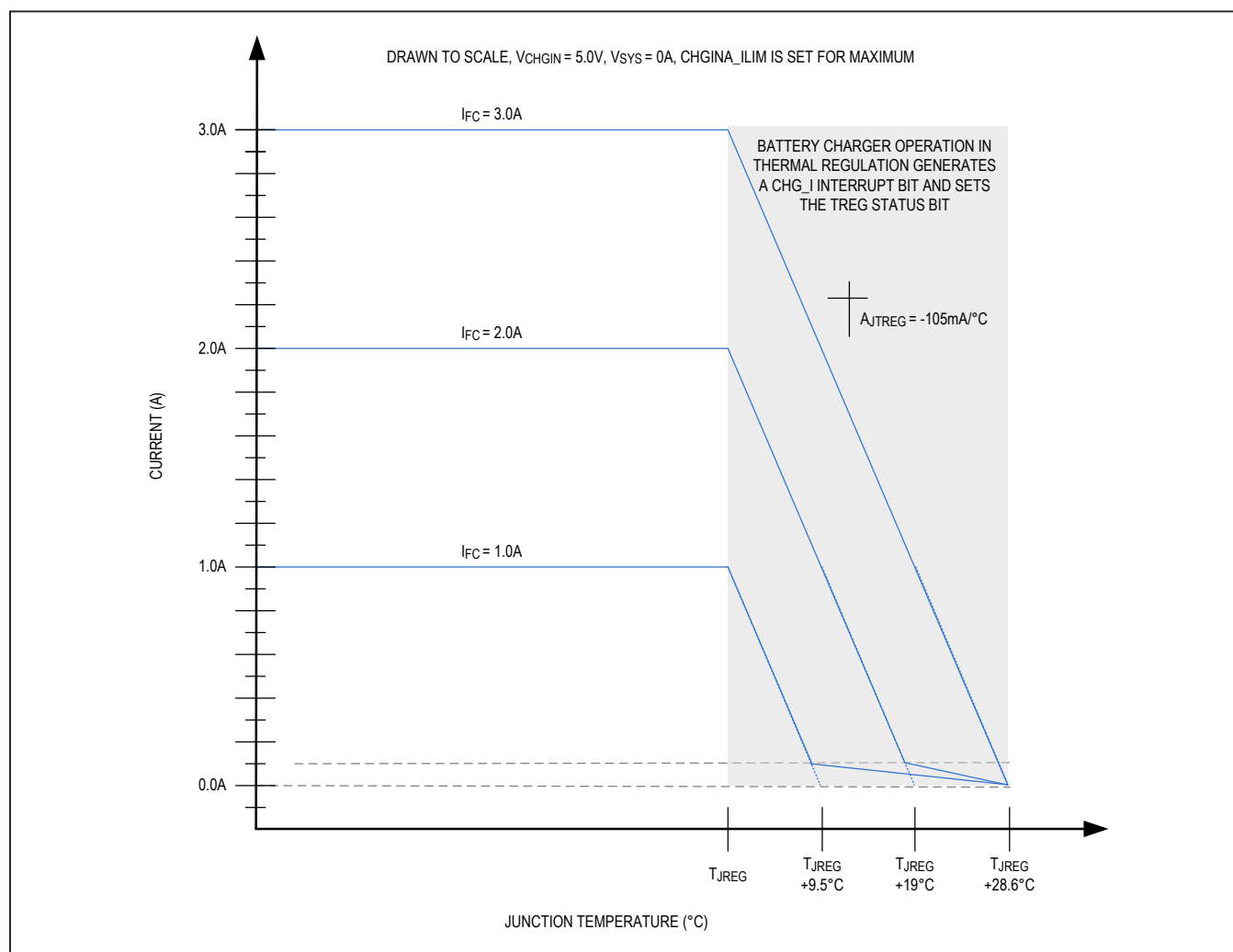
Figure 8. Charge Currents vs. Junction Temperature
