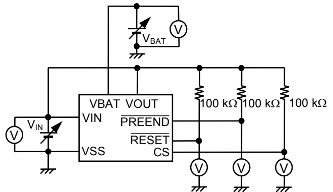
Figure 6 Test Circuit 2
