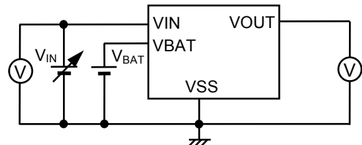
Figure 8 Test Circuit 4
