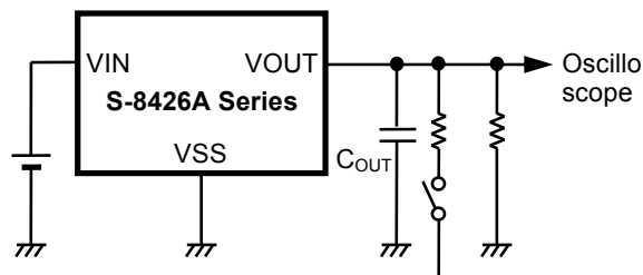
Figure 38 Test Circuit
