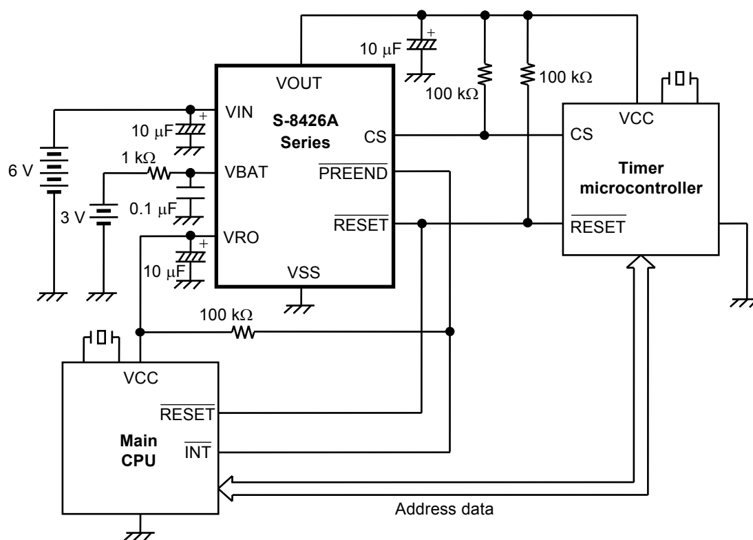
Figure 18 Application Circuit 1
