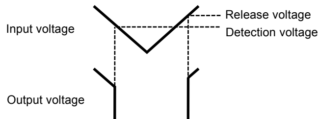
Figure 13 Definition of Detection and Release Voltages
