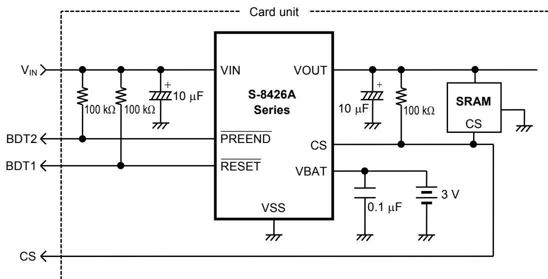
Figure 20 Application Circuit 3
