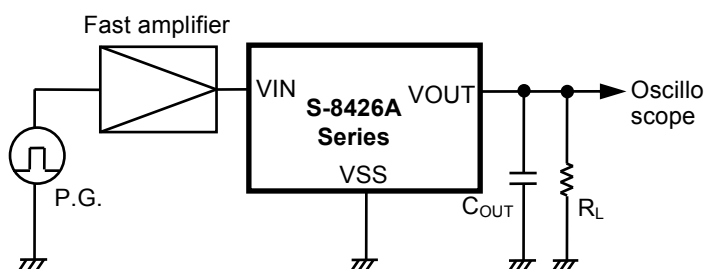
Figure 22 Test Circuit
