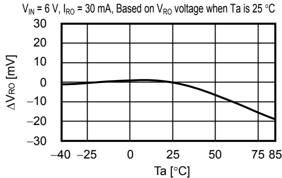
1.9 Input Stability ( V_{RO} ) Temperature Characteristics
