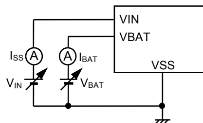
Figure 10 Test Circuit 6
