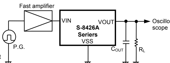
Figure 26 Test Circuit
