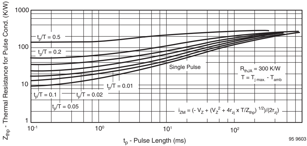
Fig. 10 - Thermal Response
