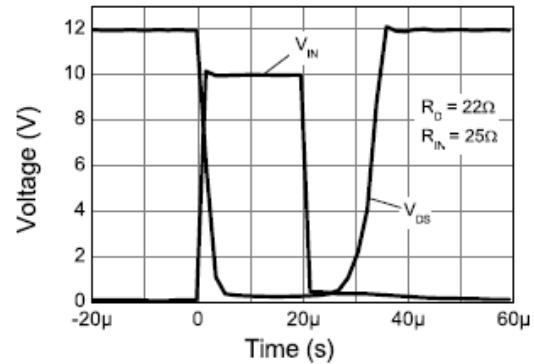
Switching Speed
