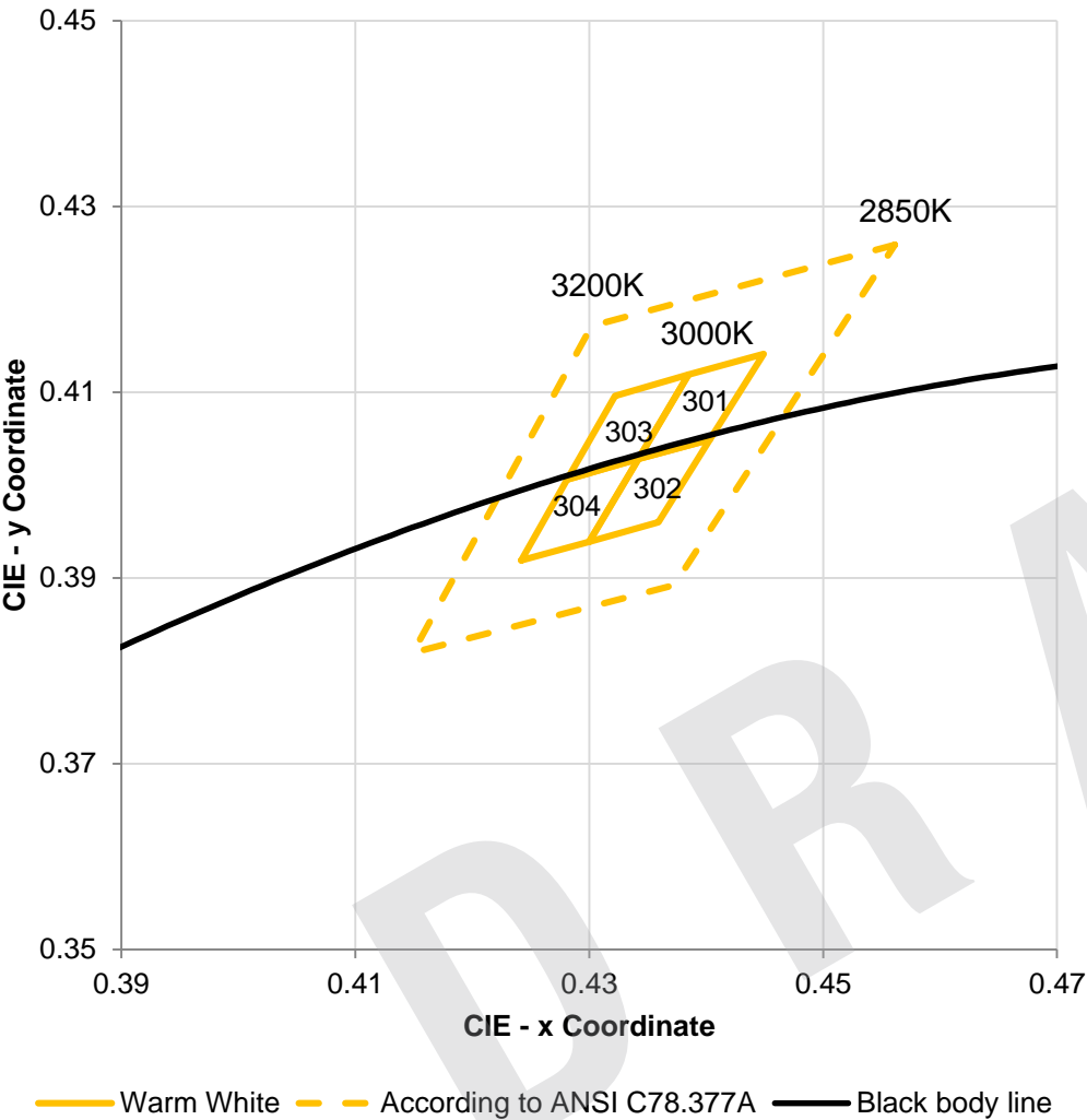
Chromaticity diagram:
