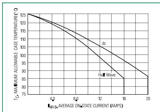
Figure 3. Current Derating
