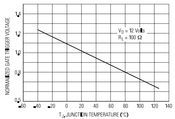
Figure 7. Gate Trigger Voltage
