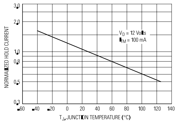
Figure 8. Holding Current
