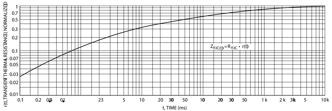
Figure 5. Thermal Response
