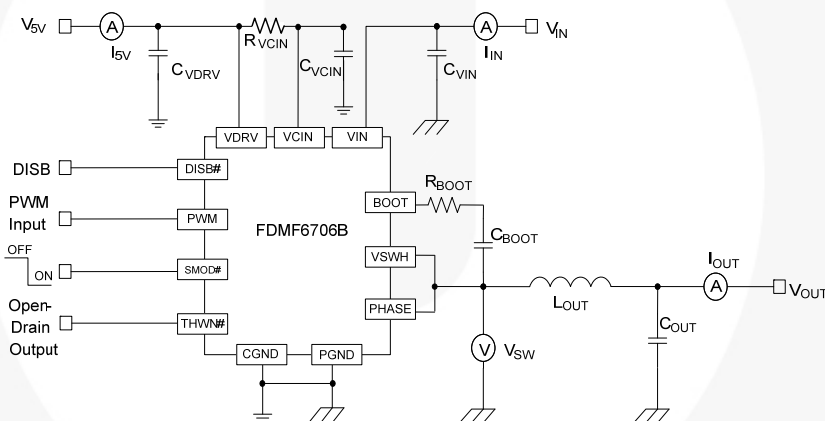
Figure 27. Block Diagram With V_{\text{CIN}} Filter
