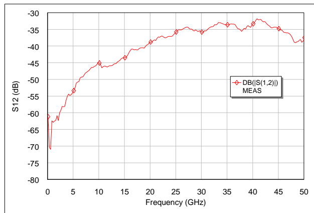
S12(dB) vs. Frequency
