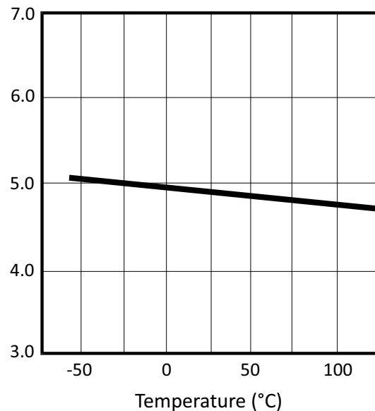
Figure 3: Power Supply Current vs. Temperature
