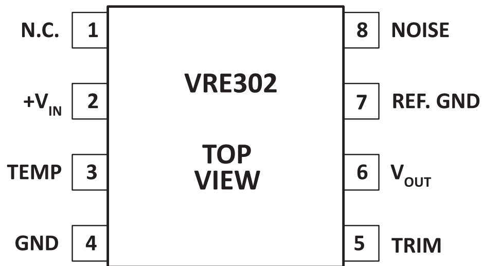
Figure 7: Pin Configuration
