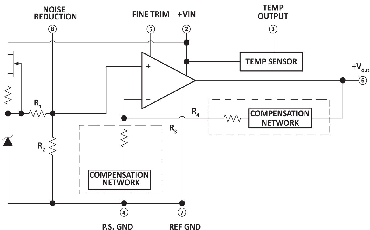
Figure 6: Block Diagram
