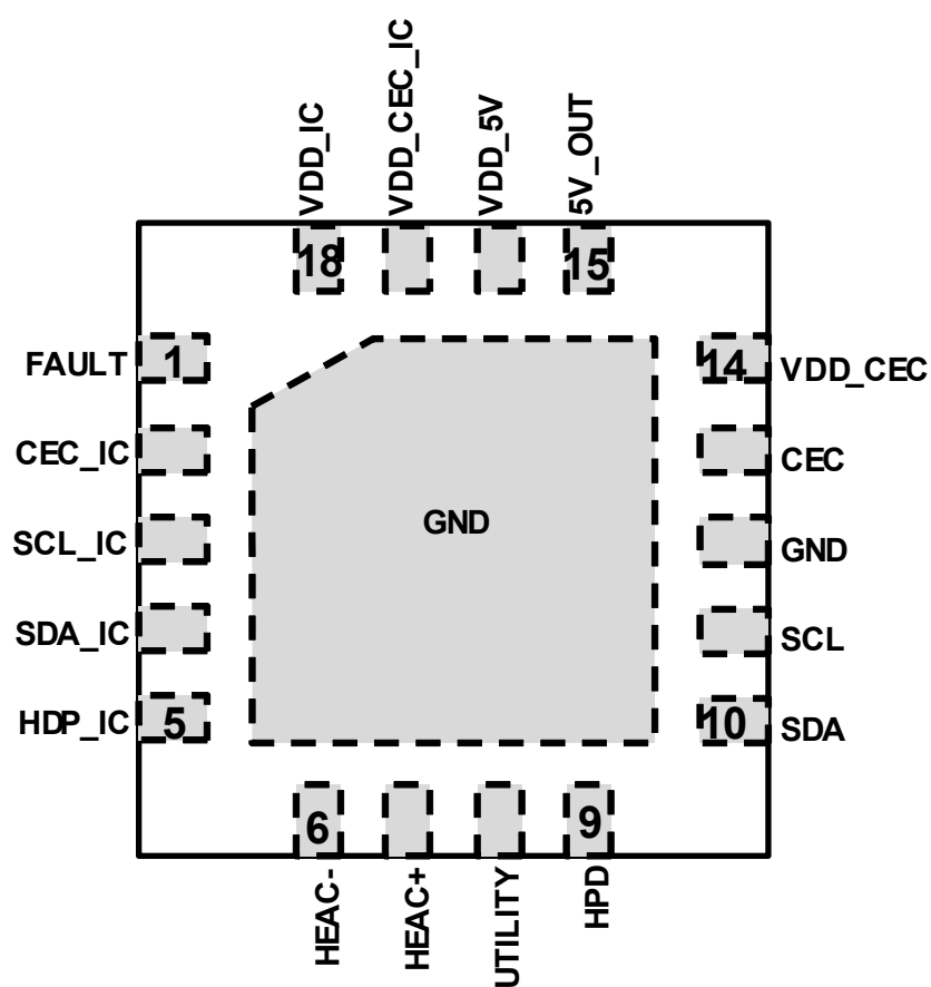
Figure 9. Pin numbering
