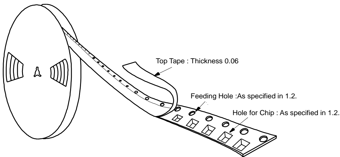
Fig.3 Taping Diagram
