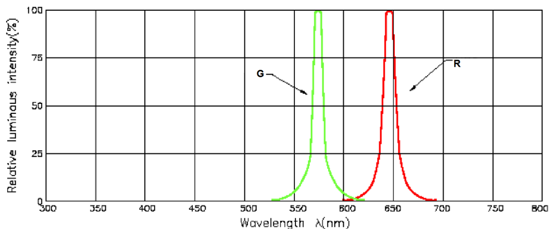
Fig. 1 Relative Luminous Intensity vs. Peak Wavelength
