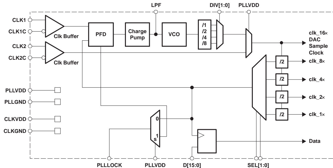
Figure 27. Clock-Generation Architecture
