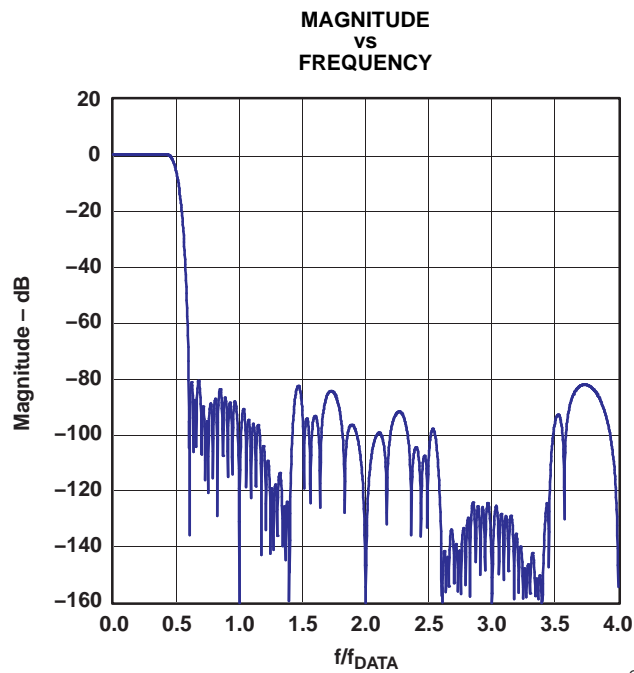
Figure 41. Magnitude Spectrum for 8x Interpolation (dB)
