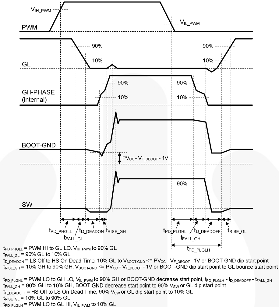
Figure 29. PWM Timing Diagram
