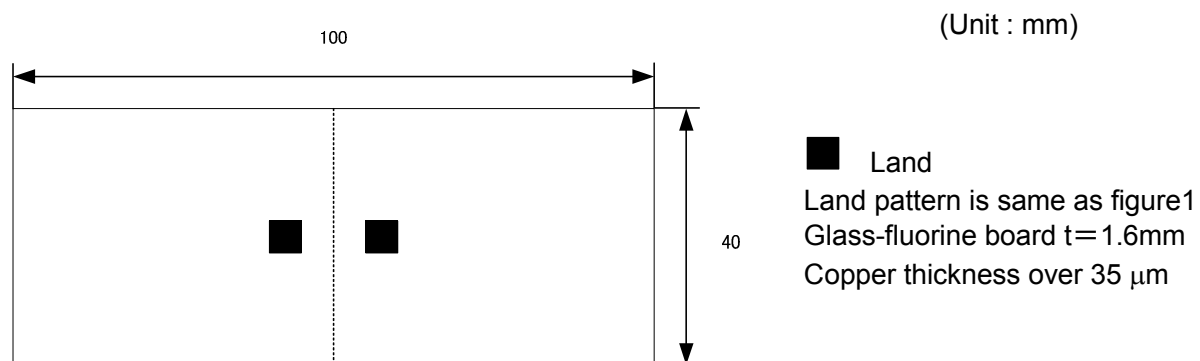
Fig. 2 Testing board
