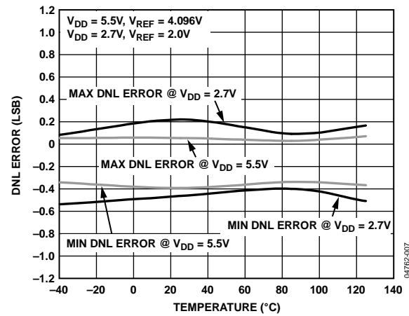
Figure 7. DNL vs. Temperature
