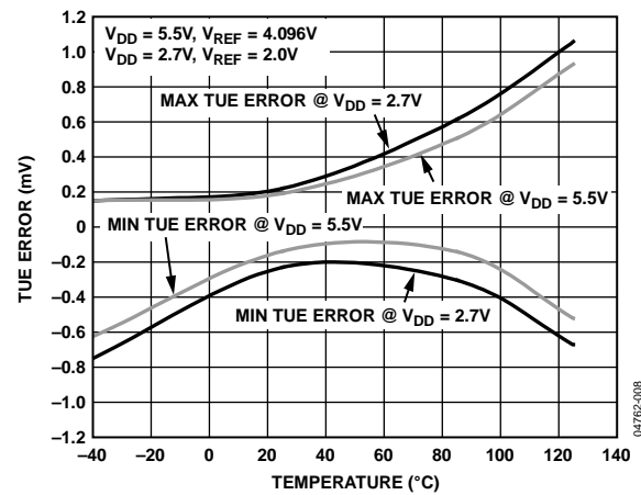
Figure 8. TUE vs. Temperature
