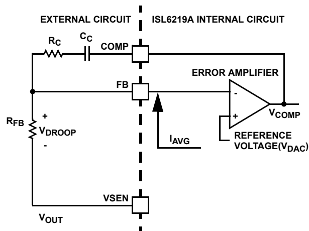
FIGURE 7. OUTPUT-VOLTAGE AND LOAD-LINE REGULATION
