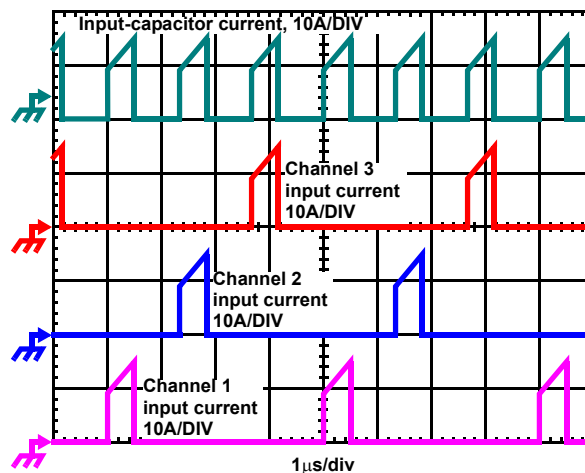
FIGURE 3. CHANNEL INPUT CURRENTS AND INPUT-CAPACITOR RMS CURRENT FOR 3-PHASE
