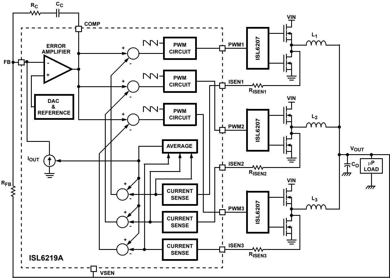
FIGURE 1. SIMPLIFIED BLOCK DIAGRAM OF THE ISL6219A
