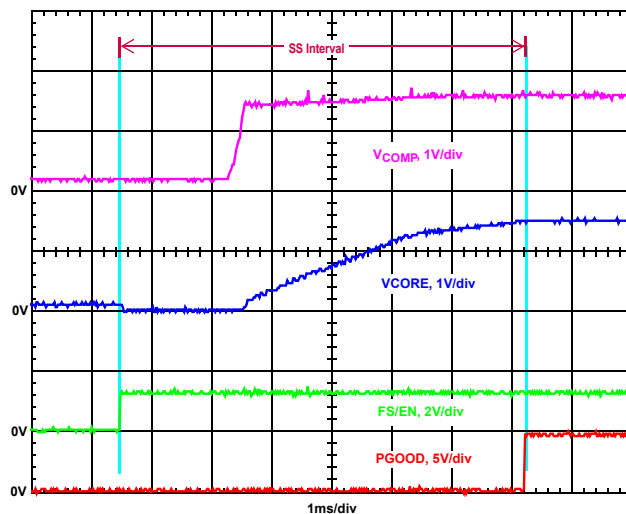
FIGURE 9. START-UP OF 3 PHASE SYSTEM OPERATING AT 300kHz
