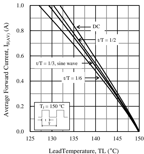
Figure 3. T_L vs. I_{F(AV)} Typical Characteristics ( V_R = 200 V)
