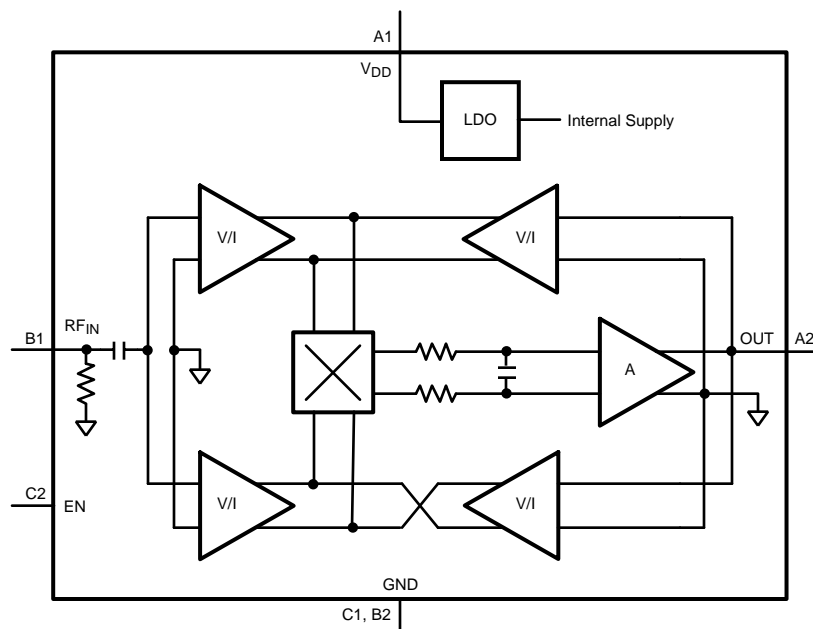
Figure 4. LMH2120
