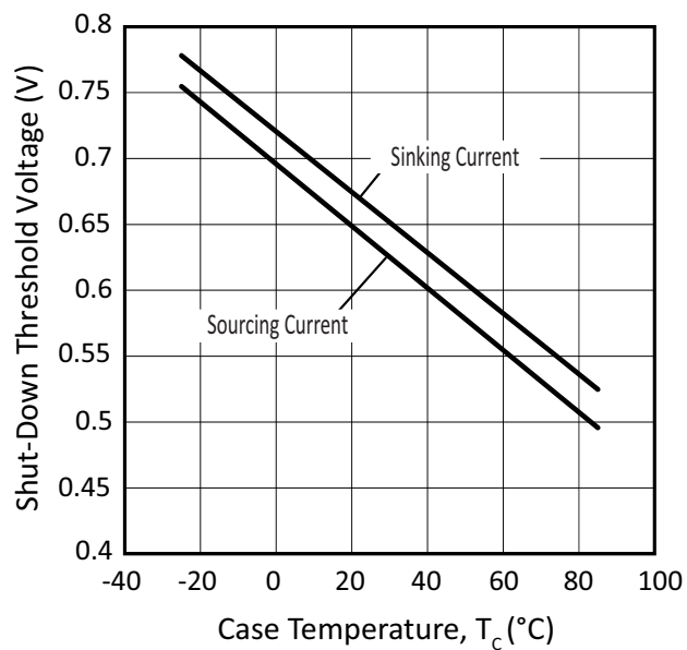
Figure 13: Shut-Down Voltage vs. Temperature
