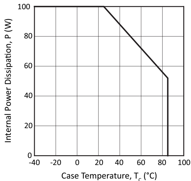
Figure 11: Power Derating
