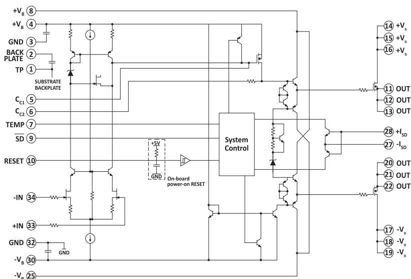
Figure 1: Equivalent Schematic
