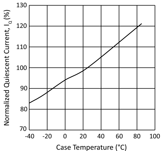
Figure 6: Quiescent Current vs. Temperature
