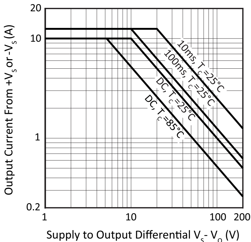
Figure 14: SOA
