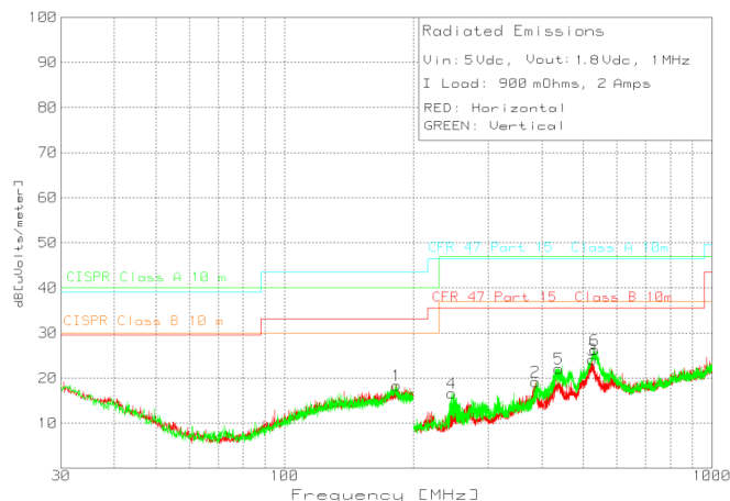
Figure 36. Radiated Emissions 5-V Input, 1.8-V Output, 2-A Load (EN55022 Class B)
