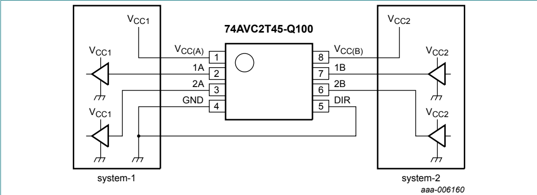
Fig. 7. Unidirectional logic level-shifting application
